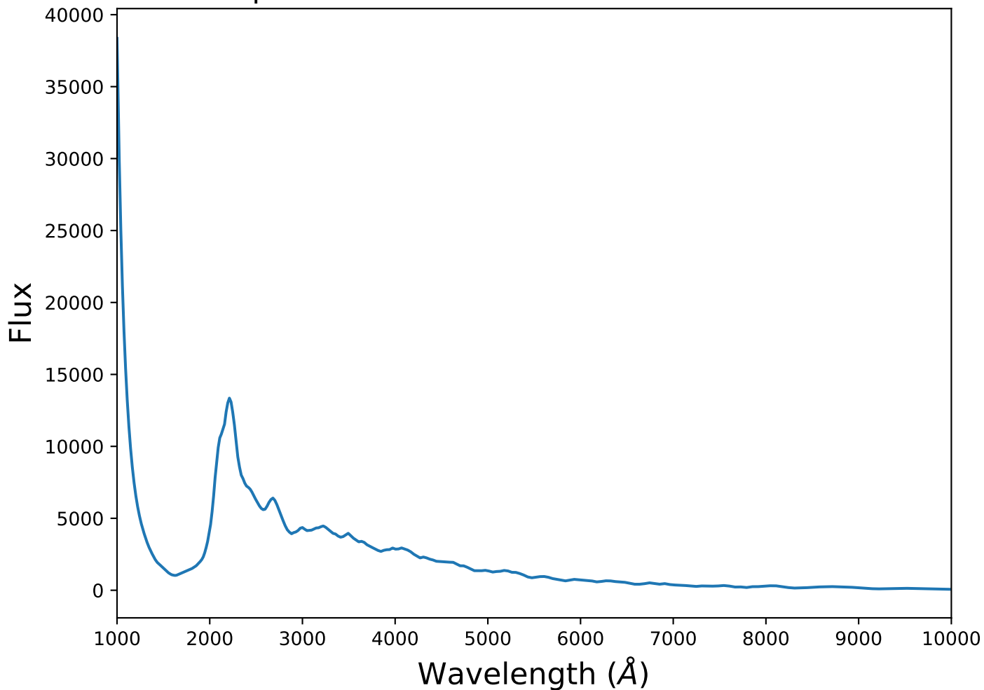
Spectrum 7 for transient SNIa at z=0.47
